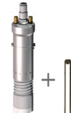
POT, blade holder 1.5 mm + blade reduction 1.5/ 0.63 mm (5003138)
