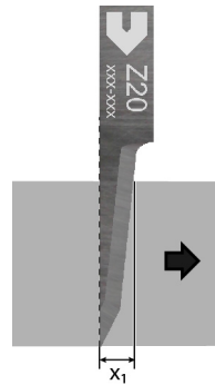
Oscillating blade – pointed
