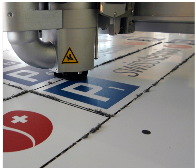
Preprinted Dibond routed with Zünd G3 2XL-3200.
